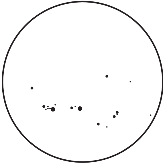
Fig 1. Sunspots at the last Solar Maximum in Cycle 24, recorded April 2014.
