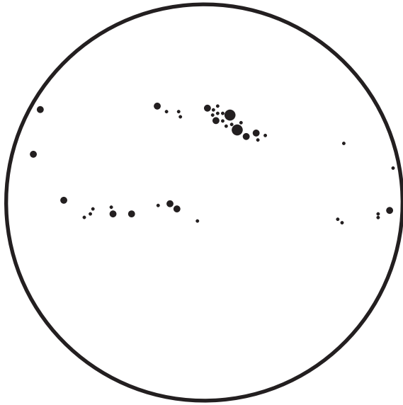
Fig 3. Sunspots at the Cycle 23 Solar Maximum, recorded November 2001.
